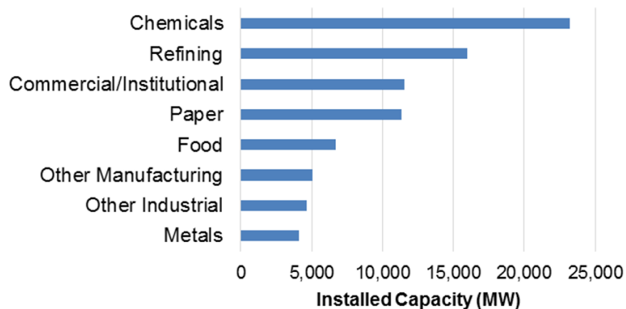
Figure I-3: Existing CHP Capacity in the United States by Facility Type 18
