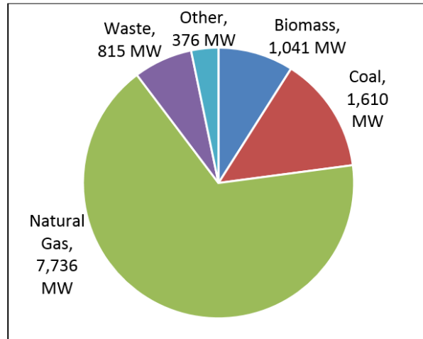
Figure II-4: Existing Commercial CHP Capacity by Fuel Class 37
