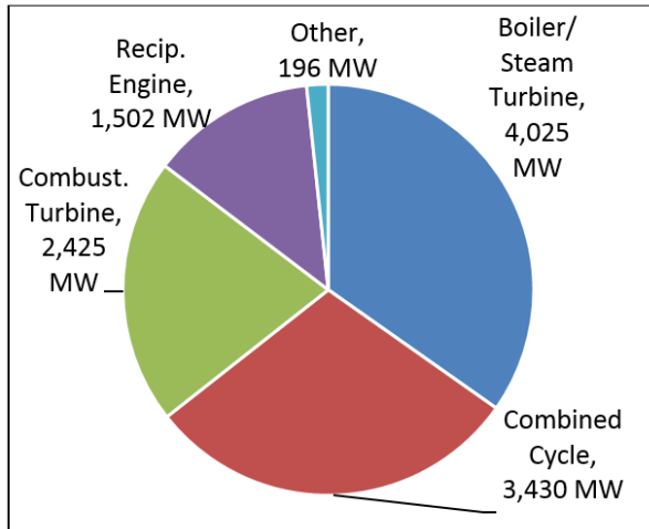
Figure II-3: Existing Commercial CHP Capacity by Prime Mover 36
