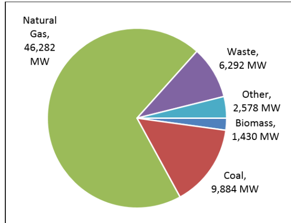
Figure II-2: Existing Industrial CHP Capacity by Fuel Class 25 (66,465 MW)
