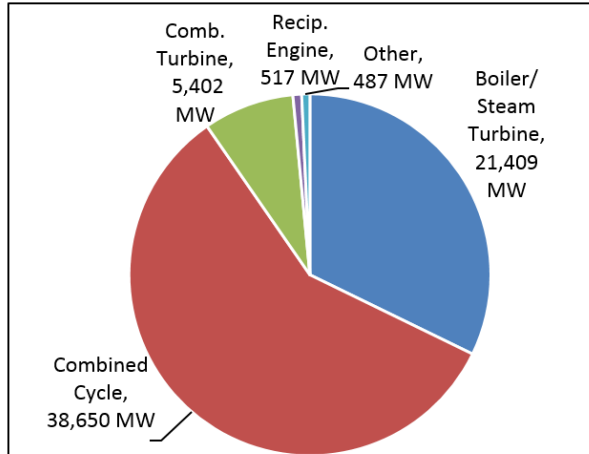
Figure II-1: Existing Industrial CHP Capacity by Prime Mover 24 (66,465 MW)
